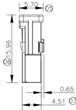
Dimensions/mm
